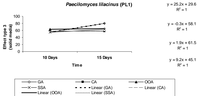
Fig.1 Linear regression curves for effect type 3 on solid agar media supplemented with gelatin (GA) casein (CA), olive oil (OOA) and starch (SSA) against eggs of Oxyuris equi at 10 and 15 days of interaction.
