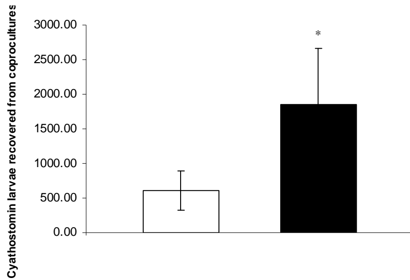
Fig. 2 Mean number and standard deviation (bar) of cyathostomin larvae recovered from coproculture of the group treated with the crude enzymatic extract of \square Pochonia chlamydosporia (VC4) and the control \blacksquare , after 8 days. Asterisk denotes significant difference ( p < 0.01 ) between the fungus-treated group and the control - Tukey's test at a 1% probability level.
