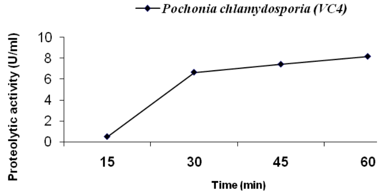
Fig. 2 – Proteolytic activity of the fungal extracts of Pochonia chlamydosporia (VC1 and VC4) at different incubation times (15, 30, 45 and 60 minutes).
