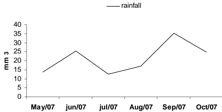
Fig.5 Monthly rainfall (mm 3 ) recorded from May to October 2007, Viçosa – MG- Brazil.
