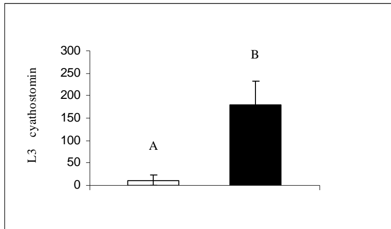
Fig.1 Mean number of non-predated cyathostomin infective larvae (L 3 ) recovered in 2% water-agar by the Baermann method at the seventh treatment day after interaction with the fungal isolate \square Duddingtonia flagrans (AC001) and group control \blacksquare . Lines on Bars represent standard deviation. Means followed by at least one common capital letter (A) in the row are not significantly different by the Tukey's test at a 1% probability level.
