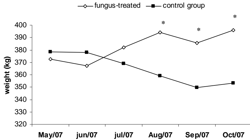
Fig.6 Monthly means of weight (kg) of fungus-treated horses and control from May to October 2007, Viçosa – MG- Brazil. Significant difference ( p < 0.01 ) between the treated group and the control denoted by asterisk-Tukey test.
