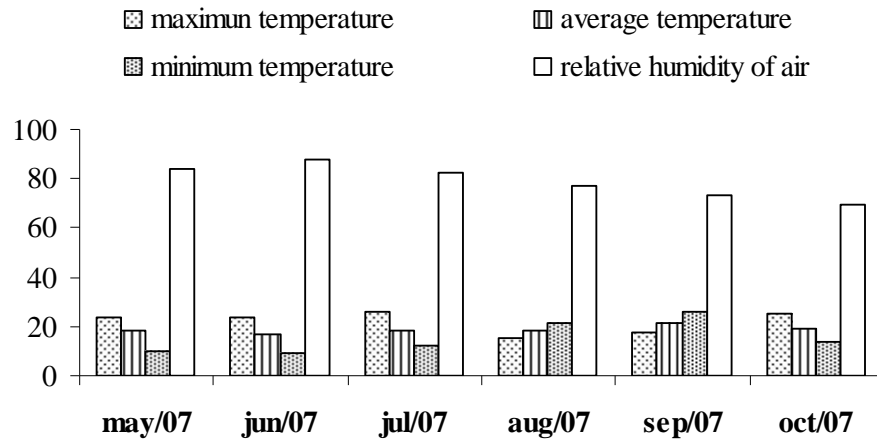
Fig.4 Averages of maximum, average and minimum monthly temperatures (°C) and air relative humidity (%) recorded from May to October 2007, Viçosa – MG- Brazil.
