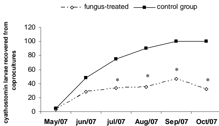
Fig.2 Mean monthly number of cyathostomin larvae recovered from coproculture of fungus-treated horses and control group collected from May to October 2007, Viçosa – MG – Brazil. Significant difference ( p < 0.01 ) between the treated group and the control denoted by asterisk- Tukey test.
