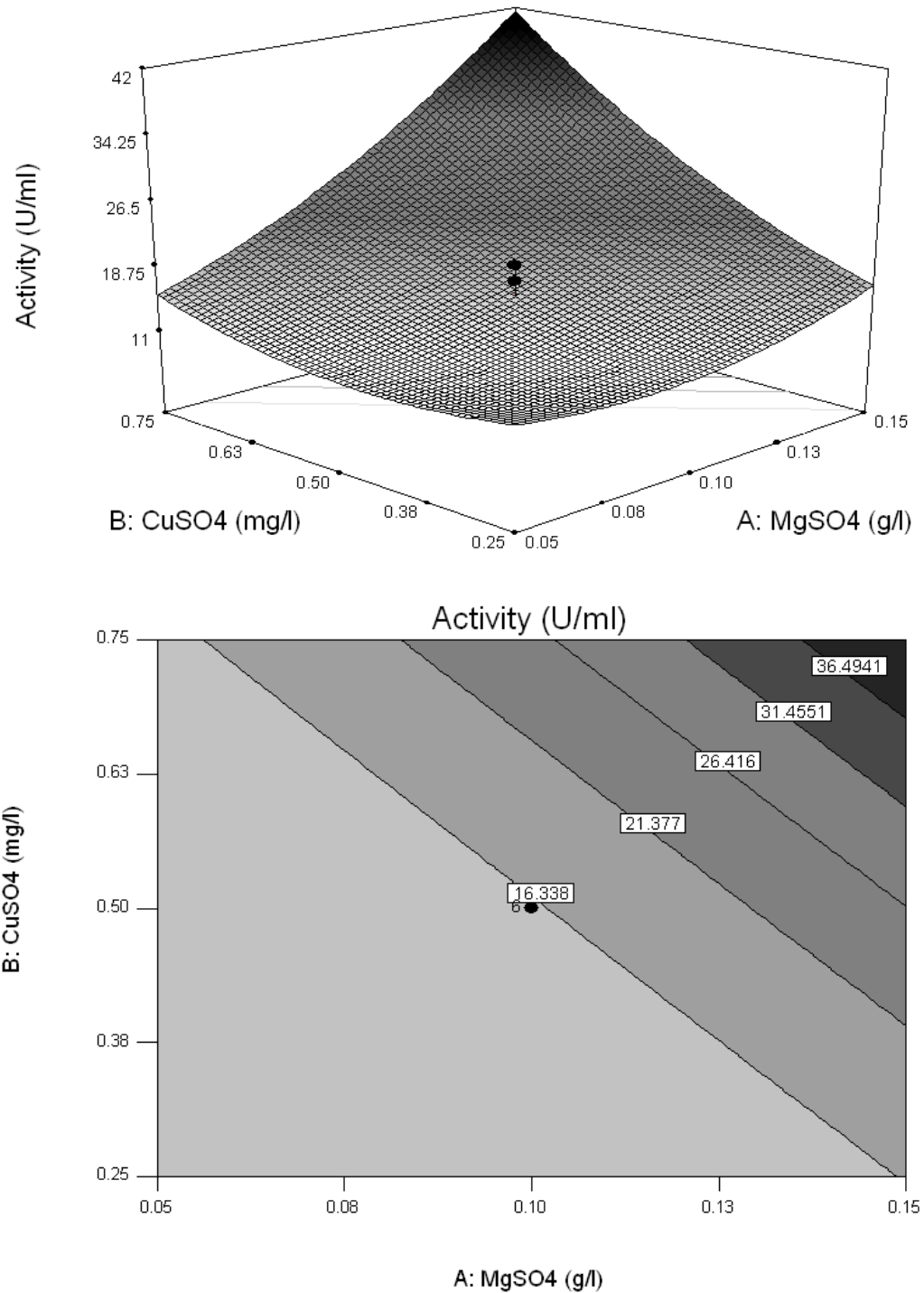
Fig. 1 Response surface curve (RSM) and contour map of the protease production by Duddingtonia flagrans (AC001) and the interaction between the variables MgSO 4 and casein (a); CuSO 4 and casein (b); MgSO 4 and CuSO 4 (c).
