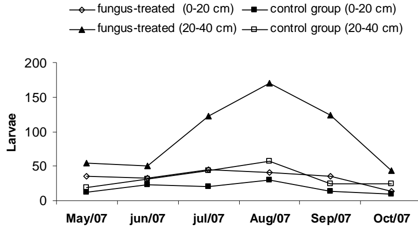
Fig.3 Monthly counts of number of infective nematode larvae per kilogram of dry matter recovered from pastures of fungus-treated horses and control collected in sampling distances up to 20 cm and 20-40 cm from fecal pats, from May to October 2007, Viçosa – MG- Brazil.
